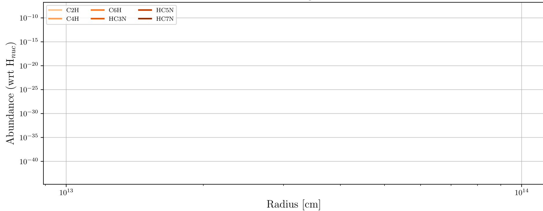
Particle 57990 - Daughter Molecules
